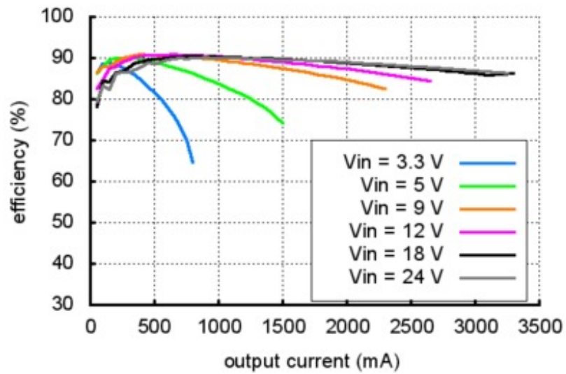
Pololu S18V20F9 Regulator Efficiency (Vout = 9 V)
