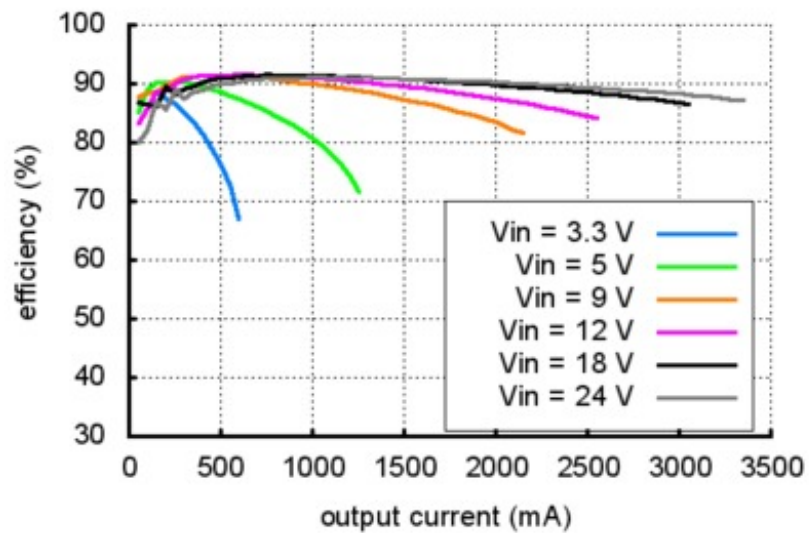
Pololu S18V20F12 Regulator Efficiency (Vout = 12 V)
