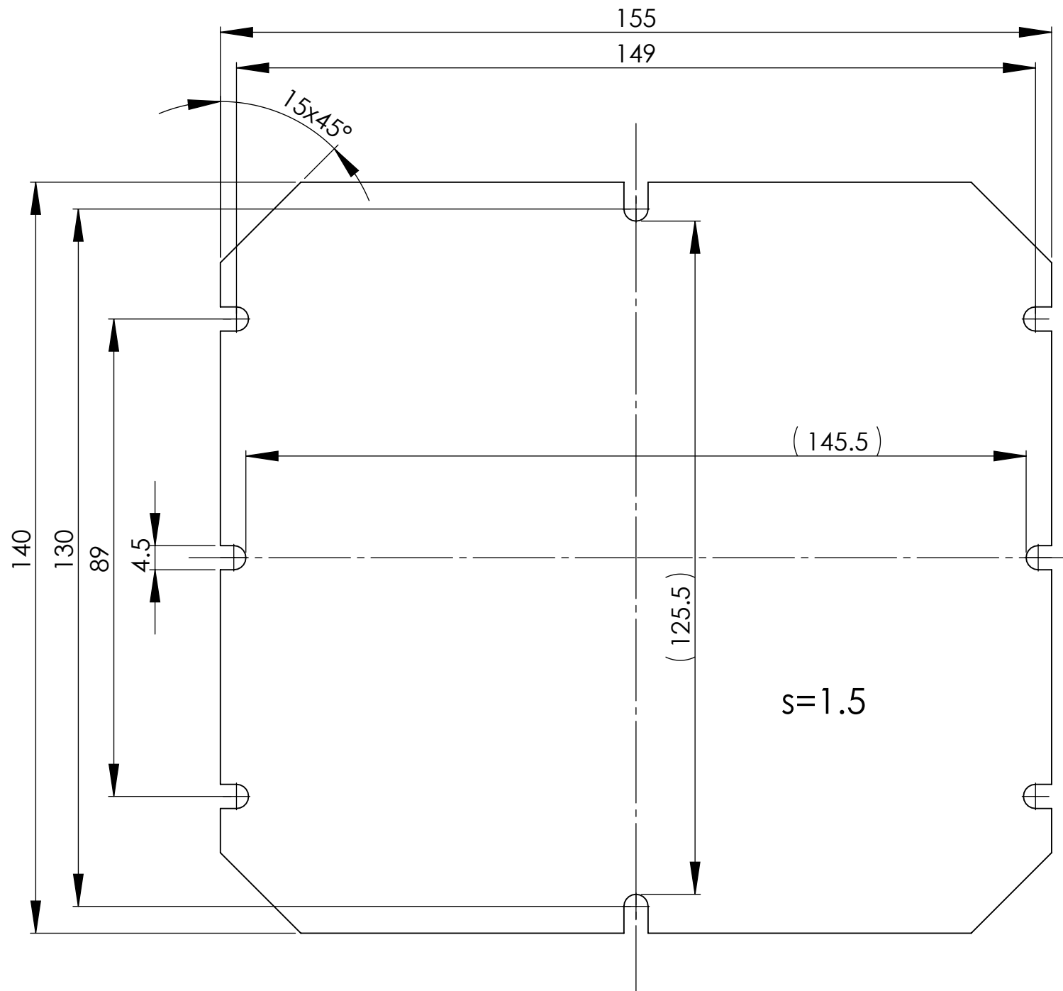
FIBOX MP2016
