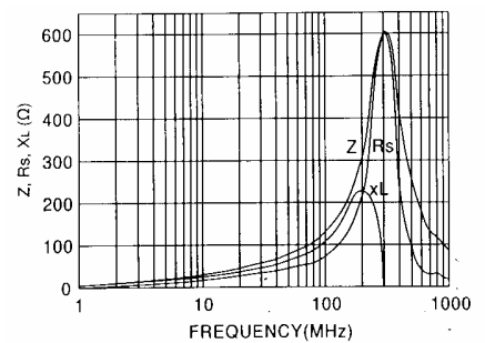
FFI55.1x15x12.7
