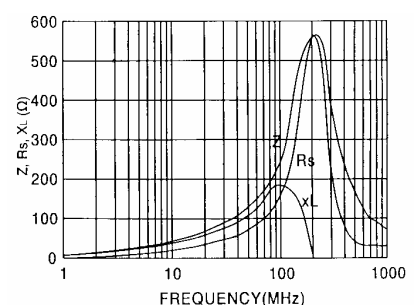
FFI76.2x28.5x12.7
