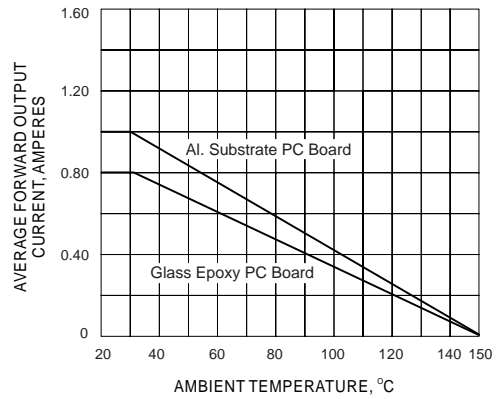
DERATING CURVE FOR OUTPUT RECTIFIED CURRENT
