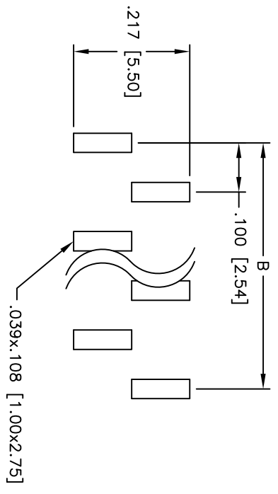
PCB LAYOUT
